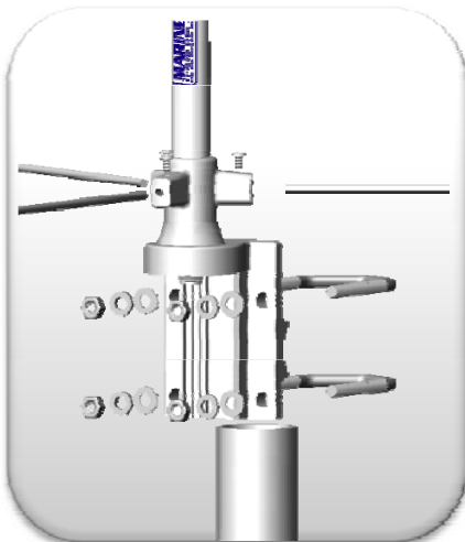
MULTI BRACKET FRONT
