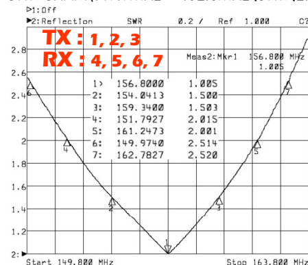
SWR CHART(149.9MHz ~ 162.8MHz<SWR<2.5)
